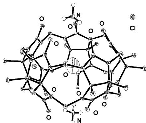
Figure 1. Crystal structure of \text{MeCuc5} \cdot 2\text{NH}_4\text{Cl} \cdot 4\text{H}_2\text{O} . The O atom of the cavity water molecule has an occupancy of 0.47. One of the external water molecules (not shown) has an occupancy of 0.28; with these values the structure converged to give R_1 = 0.044 .
